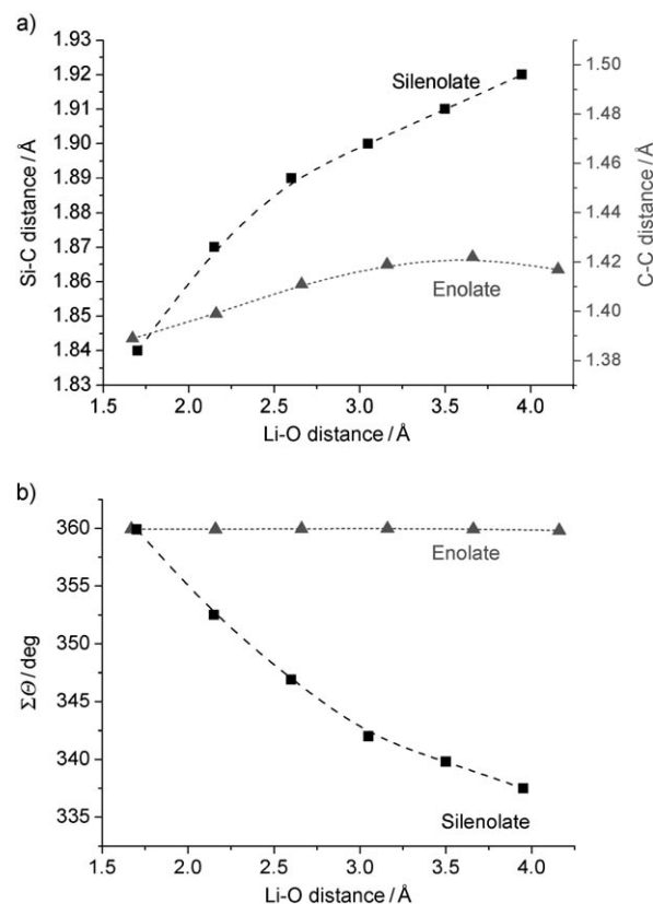
Figure 4. a) Calculated Si–C bond lengths for 1a and C–C bond lengths for 7 versus Li–O distance. b) Calculated sum of bond angles around the \alpha -E atom (for silenolate 1a and enolate 7 versus Li–O distance).
